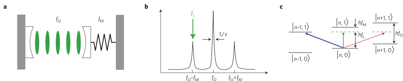
Figure 1 | Resolved-sideband cooling of an optomechanical resonator. a , Fabry-Pérot optical cavity with one mirror attached to a mechanical resonator. b , Optical cavity excitation spectrum in the resolved-sideband limit. Laser illumination (green arrow) is tuned to lower sideband. c , Energy level diagram for sideband-cooling. |n, m\rangle represents mechanical resonator phonon state n with optical cavity photon state m . Laser transition at f_L (green arrow) is accompanied by strong transitions where one phonon is absorbed to generate a cavity photon (blue arrow), cooling the resonator. Transitions where one phonon is emitted (red arrow) are very rare.
