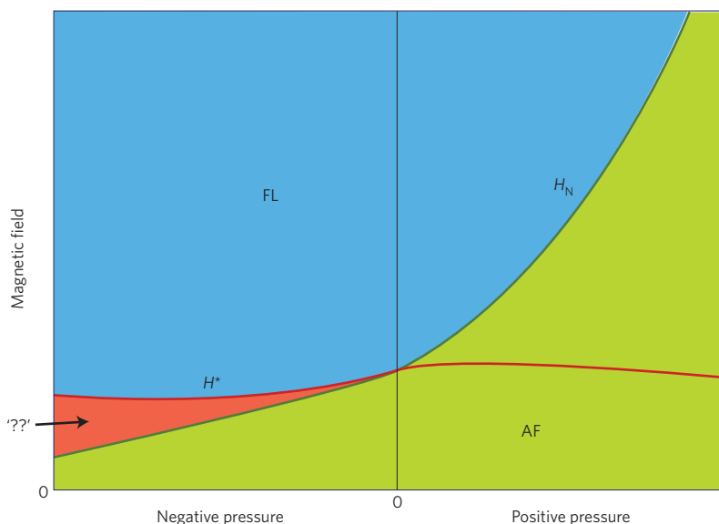
Figure 1 | Suggested phase diagram of \text{YbRh}_2\text{Si}_2 as a function of chemical pressure and magnetic field. H^* is associated with a reconstruction of the Fermi surface and H_N with the onset of Néel magnetic order. The coincidence of H^* and H_N for stoichiometric \text{YbRh}_2\text{Si}_2 apparently does not hold under chemical pressure. Most intriguing is the new, possibly non-Fermi-liquid phase (marked as '??') that is revealed at negative pressure.
