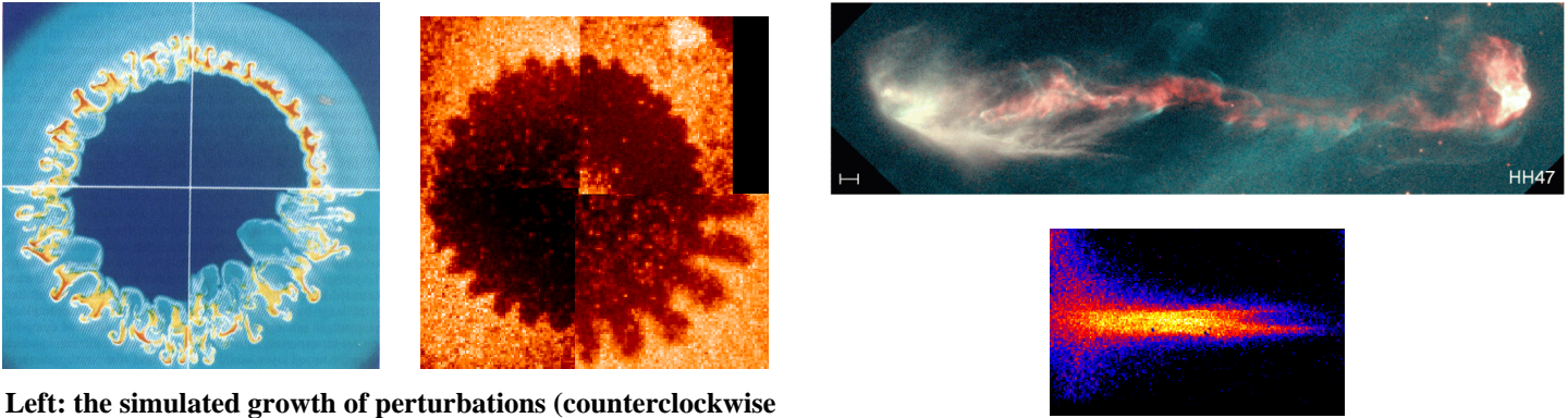
Top: the Herbig-Hero object HH47, a galactic radiative jet in interstellar space. Bottom: Experimental radiating jet formed by colliding plasmas on the Nova laser.
