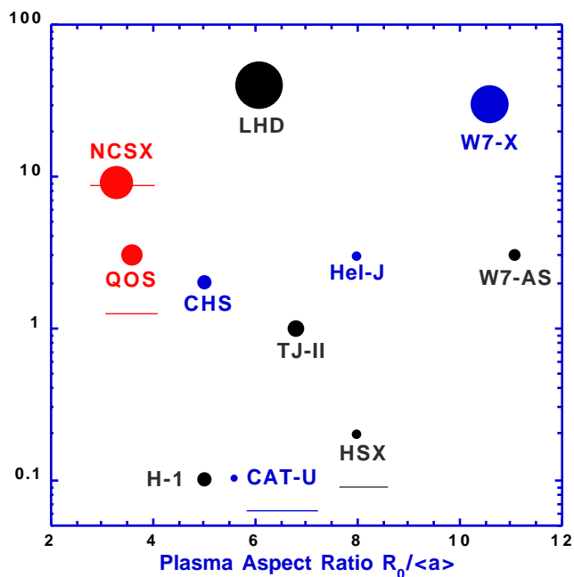
Fig. 2. Comparative sizes and heating powers for the world stellarators.
