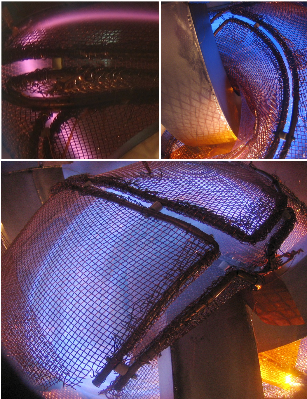
Fig. 2. Visualization photographs taken with 4 second exposure on a digital camera. (a) A glowing field line is plainly visible intersecting the conducting boundary prior to alignment. (b)(c) Large outer surfaces glowing inside the conducting boundary without intersecting it.
